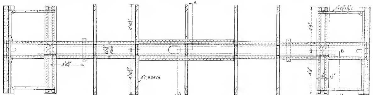
Underframe of the Santa Fe Tank Car.
